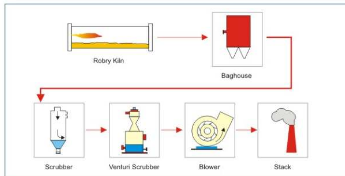
Air Pollution Control Device (APCD) installed at hot mix plant
